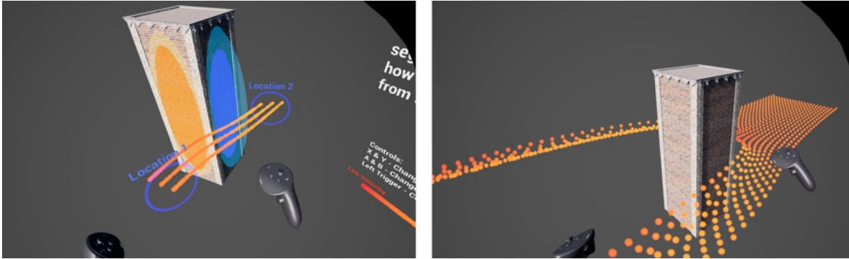
Figure 1: VR environment used for wind simulation. left) Comparison of wind velocity and pressure at two locations around a building. right) Visualization of wind flow between buildings using particle-based streamlines.
